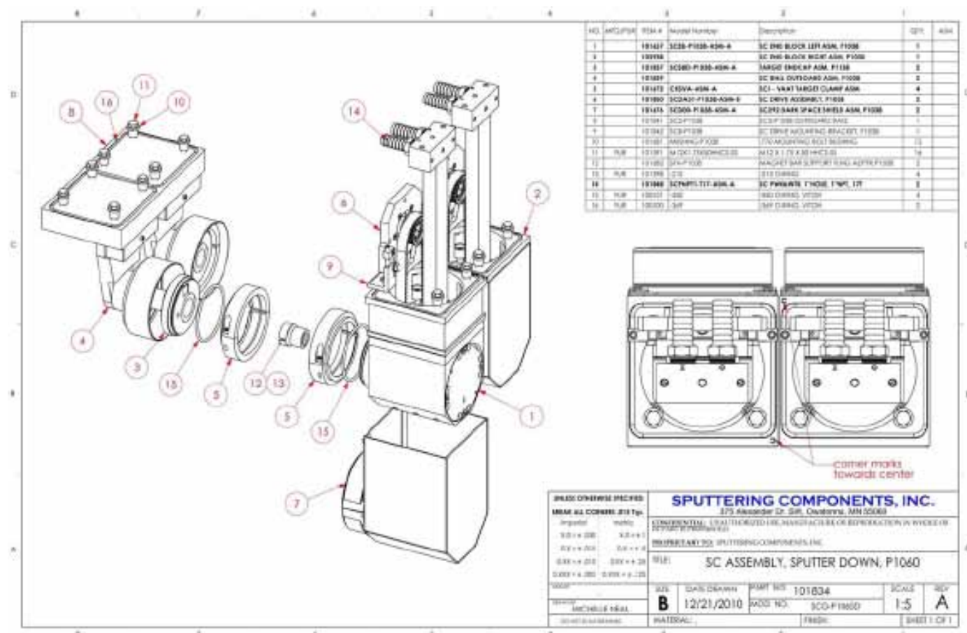
SCI end block upgrade kit for new generation Von Ardenne® Coaters
